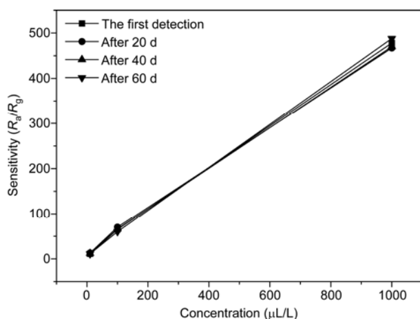
Figure 8 Sensitivities of the micro-sensors to 10, 100, and 1000 μL/L H 2 S measured up to 60 days.
